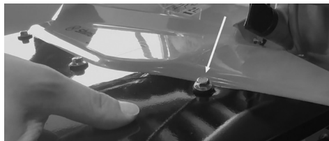
Screws corresponding to the rear support.
